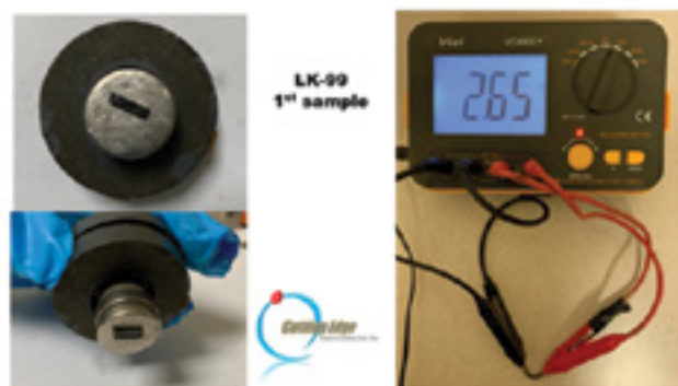
Figure 4. LK-99 sample made by solid-state reaction, according to the recipe from the Korean company [1,2]. Note that it shows the ferromagnetic attraction to the magnet and metallic behavior with resistance 2.65 ohm.
