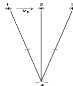
Figure 11. The past (1), verily (2) and the future (3) positions of astronomical object. Portion of light emitted by object in position (1) reaches observer (4) many years after. During this time the object that moves perpendicular to observer with speed v_t , moves to position (2). If at the moment of record portion of light were emitted for point of observation it would meet object in point (3).
