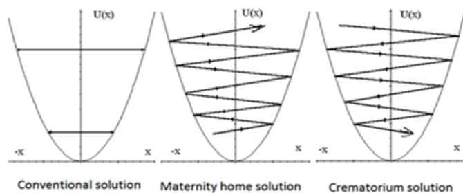
Figure 9. Solution of UQT for harmonic oscillator
