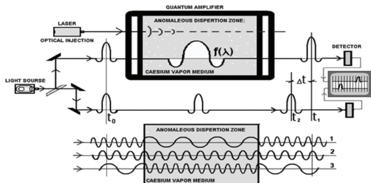
Figure 6. Experiments of L.Wang - superluminal light propagation.
