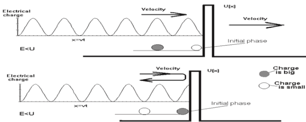
Figure 13. Illustration of the tunnel effect
