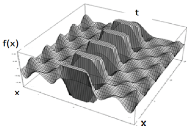
Figure 2. During the motion, the packet f(x) will appear and disappear periodically.
