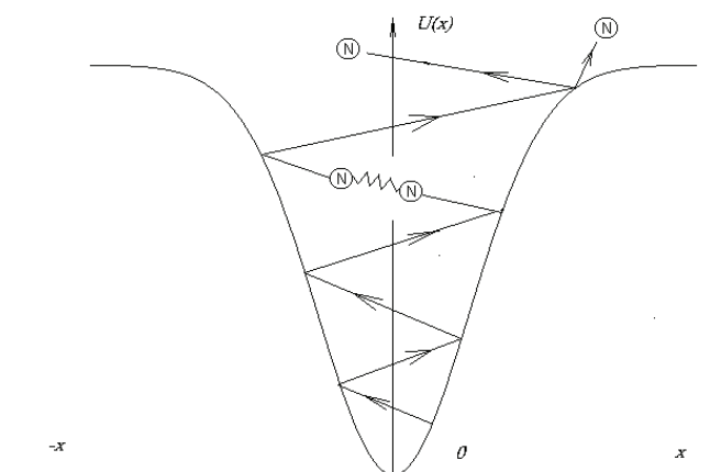
Figure 12. Oscillation of Nitrogen molecule in potential well of catalyst.
