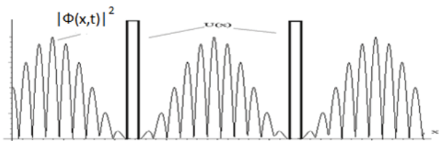
Figure 14. Illustration of the tunnel effect
