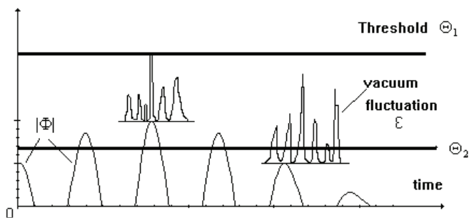
Figure 5. Quantum measurements.
