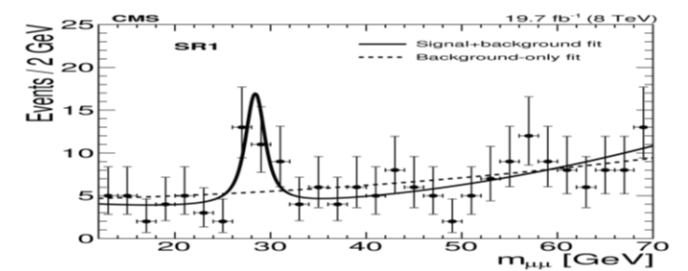
Figure 7. Peak of energy at 28GeV
