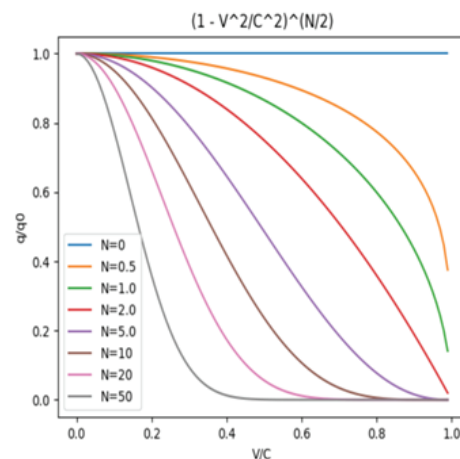
Figure 1. q/q_0 = (1 - v^2/c^2)^{N/2}
